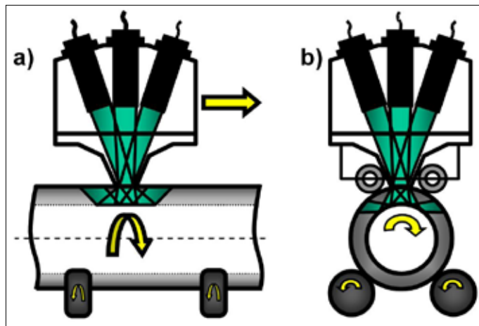
Testing principle with five ultrasonic incidence angles and helical testing traces (rotating tube, linear probe holder movement):
